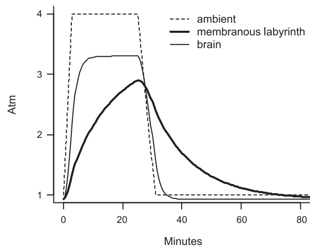
Fig. 1. Time course of gas kinetics in the brain and membranous labyrinth of the inner ear during and after a no-stop dive. Absolute ambient pressure (dashed line) and compartment gas tensions (solid lines) are shown in atm. Compartment gas tensions include a fixed contribution of 0.19 atm representing oxygen, carbon dioxide, and water vapor. Note the prolonged supersaturation of the membranous labyrinth after decompression.
